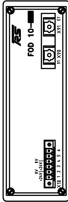
Ansicht "A" view "A"
