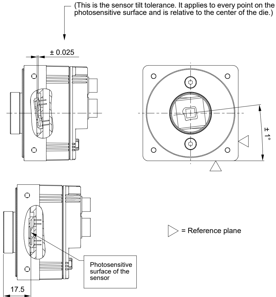
Fig. 5: Sensor Positioning Accuracy (in mm unless otherwise noted)
