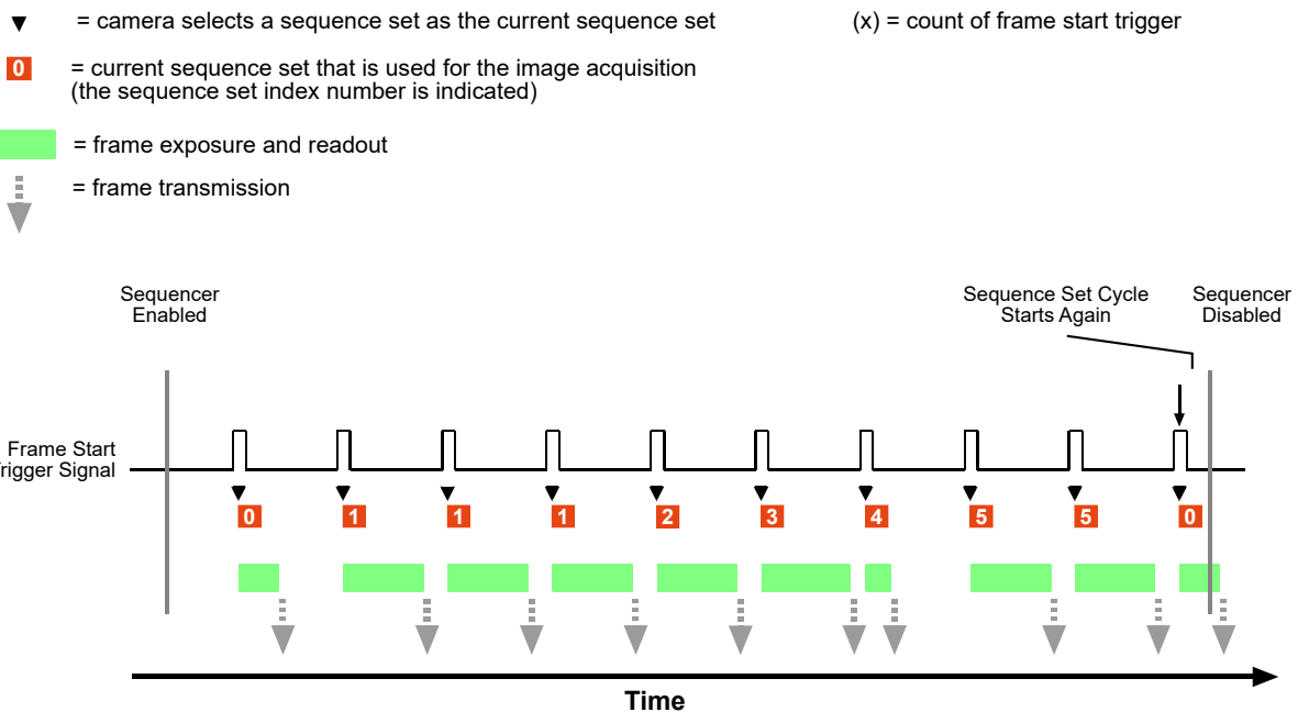
Fig. 53: Sequencer in Auto Sequence Advance Mode
