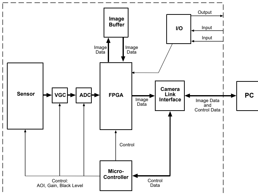
Fig. 20: Camera Block Diagram - One Tap Mode
