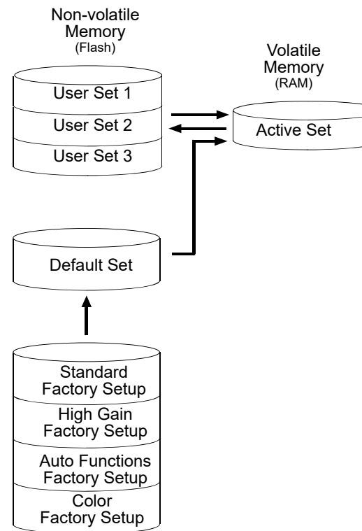
Fig. 70: Configuration Sets
