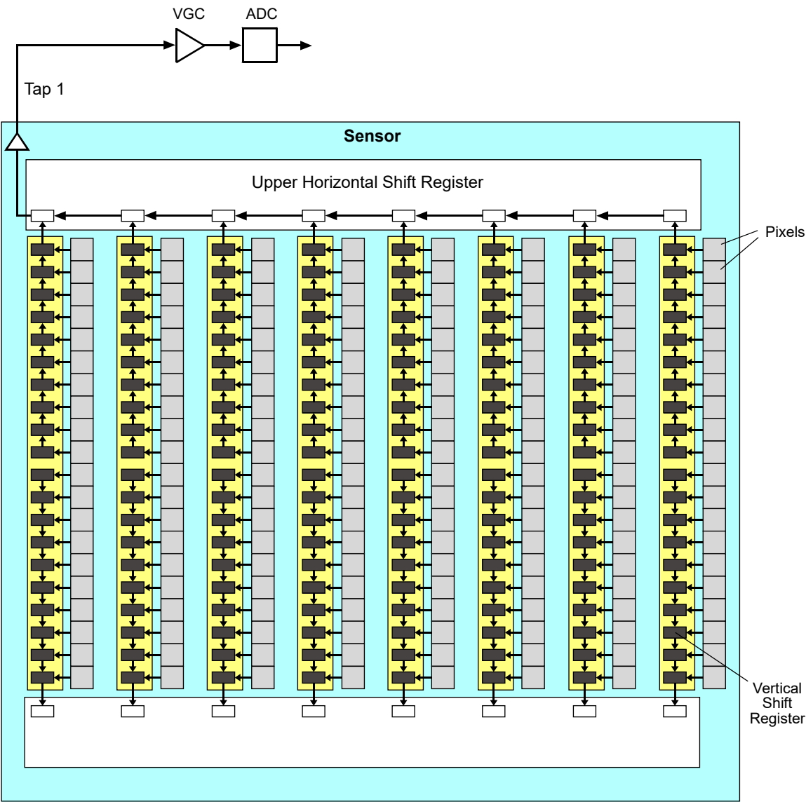
Fig. 19: One Tap Sensor Readout Mode
