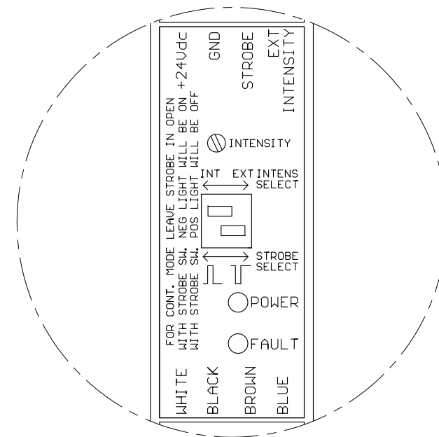
LABEL DETAIL
