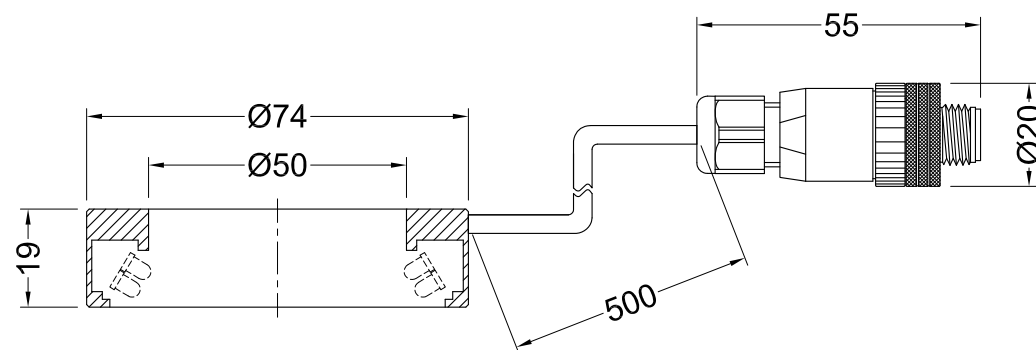
M12 X 1 MALE CONNECTOR
