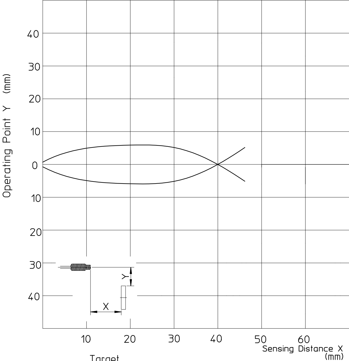
Target White at 90% reflectance (250x200mm)
