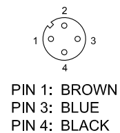
M12 X 1 CONNECTOR (FEMALE)
